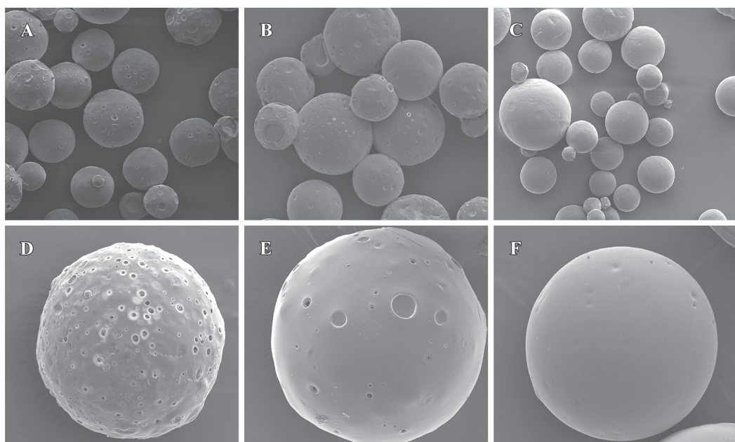
Figure 1. Scanning electron micrography of the surface morphology of IFN- \alpha 2b MS with different inherent viscosities PLGA. A (D) 0.39 dL·g ^{-1} ; B (E) 0.89 dL·g ^{-1} ; and C (F) 1.13 dL·g ^{-1} .
